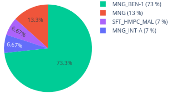
Neighbors in UMAP for 207851030093_R08C01 reference: AllIDATv2_20210804_HPAP_Sarc.xlsx (19967 cases), 0 CpGs
