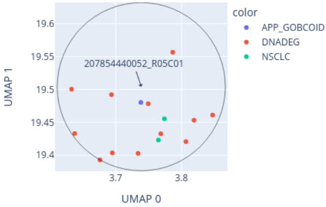
Close-up of UMAP for 207854440052_R05C01 reference: AllIDATv2_20210804_HPAP_Sarc.xlsx (19967 cases), 0 CpGs
