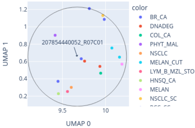
Close-up of UMAP for 207854440052_R07C01 reference: AllIDATv2_20210804_HPAP_Sarc.xlsx (19967 cases), 0 CpGs
