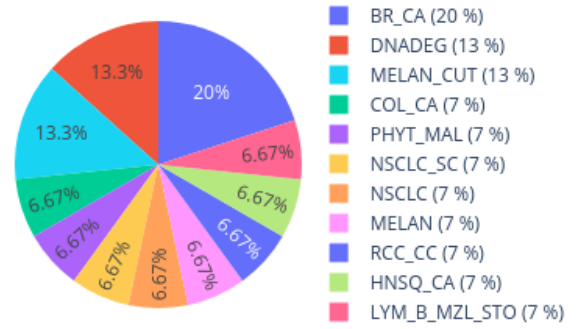
Neighbors in UMAP for 207854440052_R07C01 reference: AllIDATv2_20210804_HPAP_Sarc.xlsx (19967 cases), 0 CpGs
