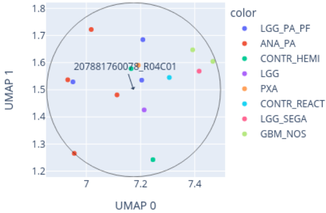
Close-up of UMAP for 207881760078_R04C01 reference: AllIDATv2_20210804_HPAP_Sarc.xlsx (19967 cases), 0 CpGs
