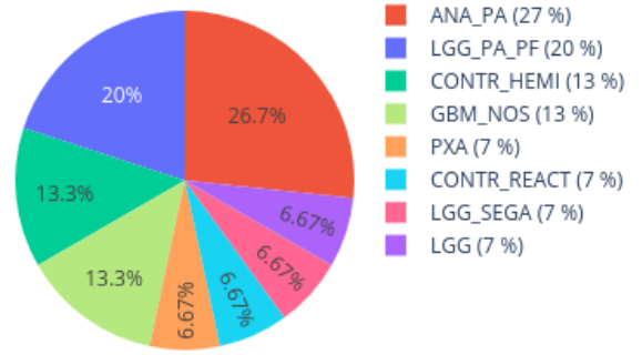
Neighbors in UMAP for 207881760078_R04C01 reference: AllIDATv2_20210804_HPAP_Sarc.xlsx (19967 cases), 0 CpGs
