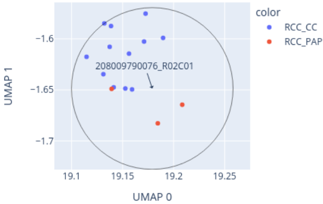
Close-up of UMAP for 208009790076_R02C01 reference: AllIDATv2_20210804_HPAP_Sarc.xlsx (19967 cases), 0 CpGs
