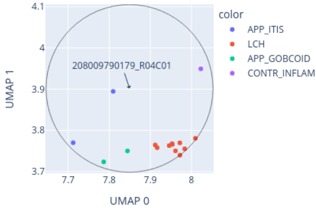
Close-up of UMAP for 208009790179_R04C01 reference: AllIDATv2_20210804_HPAP_Sarc.xlsx (19967 cases), 0 CpGs
