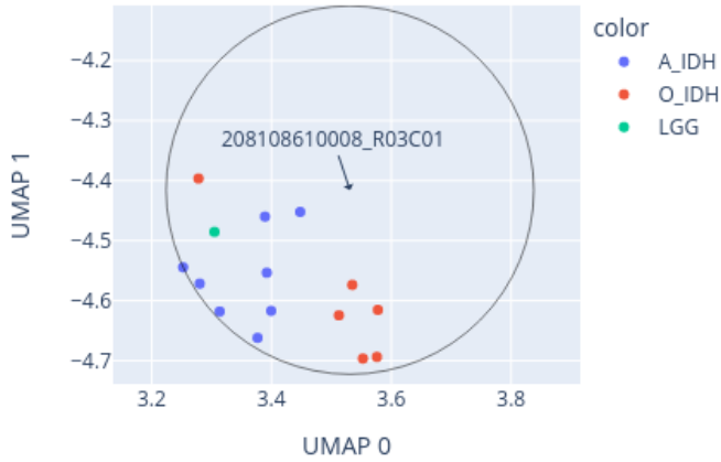
Close-up of UMAP for 208108610008_R03C01 reference: AllIDATv2_20210804_HPAP_Sarc.xlsx (19967 cases), 0 CpGs
