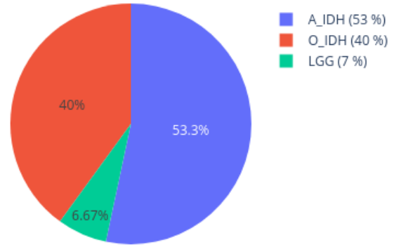
Neighbors in UMAP for 208108610008_R03C01 reference: AllIDATv2_20210804_HPAP_Sarc.xlsx (19967 cases), 0 CpGs
