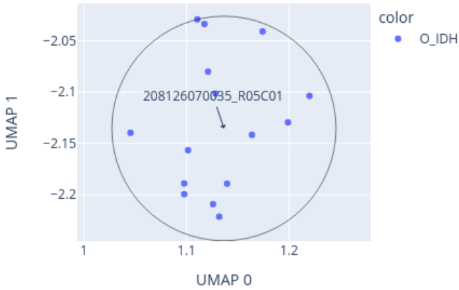
Close-up of UMAP for 208126070035_R05C01 reference: AllIDATv2_20210804_HPAP_Sarc.xlsx (19967 cases), 0 CpGs
