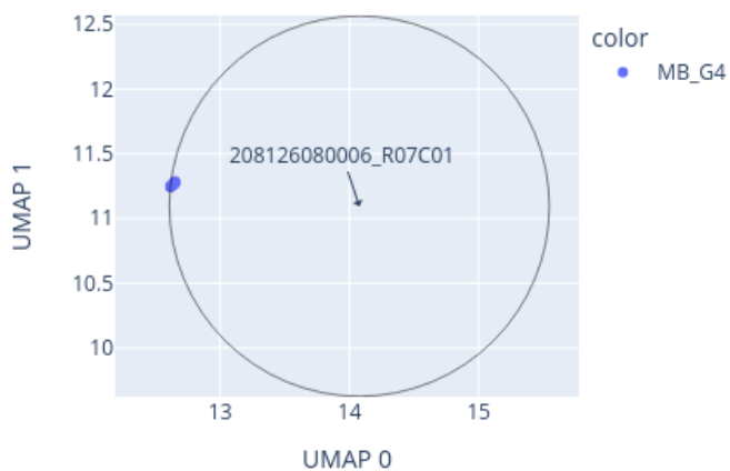
Close-up of UMAP for 208126080006_R07C01 reference: AllIDATv2_20210804_HPAP_Sarc.xlsx (19967 cases), 0 CpGs
