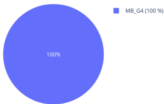
Neighbors in UMAP for 208126080006_R07C01 reference: AllIDATv2_20210804_HPAP_Sarc.xlsx (19967 cases), 0 CpGs
