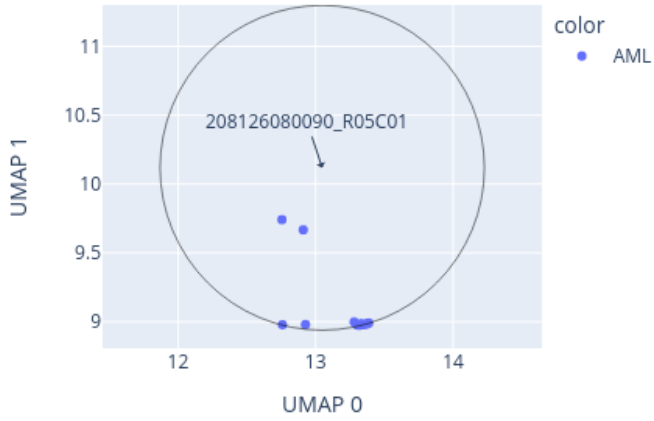
Close-up of UMAP for 208126080090_R05C01 reference: AllIDATv2_20210804_HPAP_Sarc.xlsx (19967 cases), 0 CpGs
