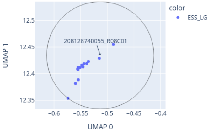
Close-up of UMAP for 208128740055_R08C01 reference: AllIDATv2_20210804_HPAP_Sarc.xlsx (19967 cases), 0 CpGs
