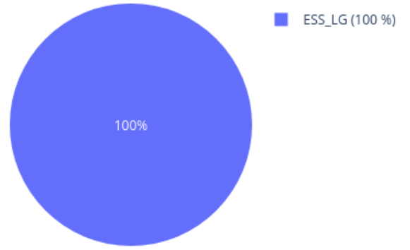
Neighbors in UMAP for 208128740055_R08C01 reference: AllIDATv2_20210804_HPAP_Sarc.xlsx (19967 cases), 0 CpGs
