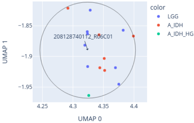
Close-up of UMAP for 208128740112_R06C01 reference: AllIDATv2_20210804_HPAP_Sarc.xlsx (19967 cases), 0 CpGs
