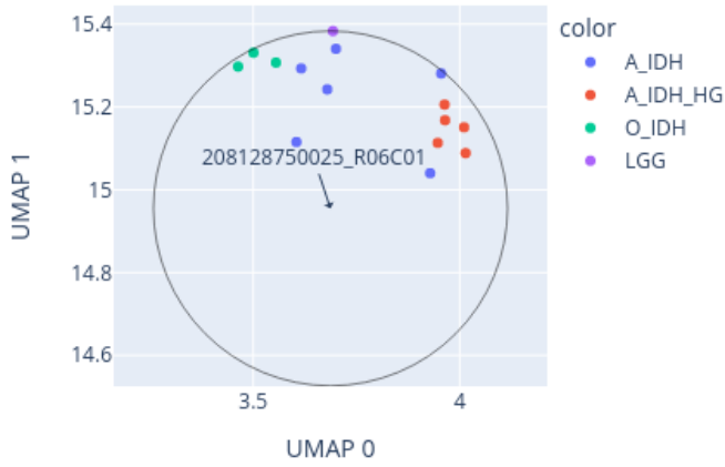
Close-up of UMAP for 208128750025_R06C01 reference: AllIDATv2_20210804_HPAP_Sarc.xlsx (19967 cases), 0 CpGs
