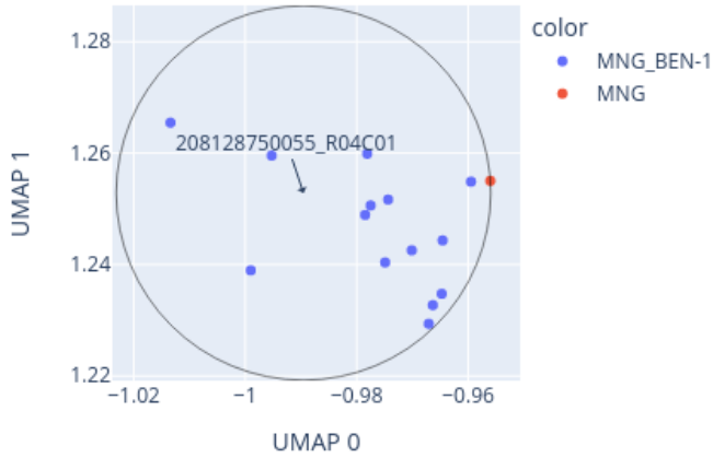
Close-up of UMAP for 208128750055_R04C01 reference: AllIDATv2_20210804_HPAP_Sarc.xlsx (19967 cases), 0 CpGs
