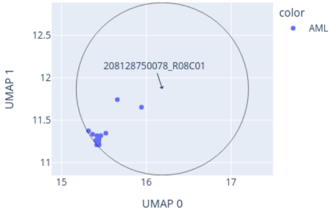
Close-up of UMAP for 208128750078_R08C01 reference: AllIDATv2_20210804_HPAP_Sarc.xlsx (19967 cases), 0 CpGs
