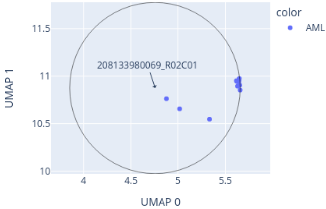
Close-up of UMAP for 208133980069_R02C01 reference: AllIDATv2_20210804_HPAP_Sarc.xlsx (19967 cases), 0 CpGs
