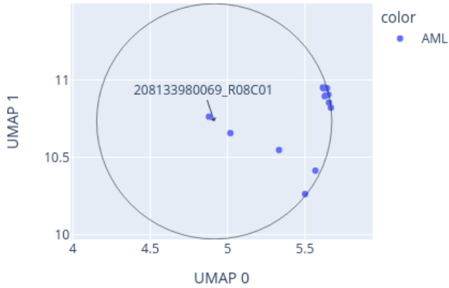
Close-up of UMAP for 208133980069_R08C01 reference: AllIDATv2_20210804_HPAP_Sarc.xlsx (19967 cases), 0 CpGs
