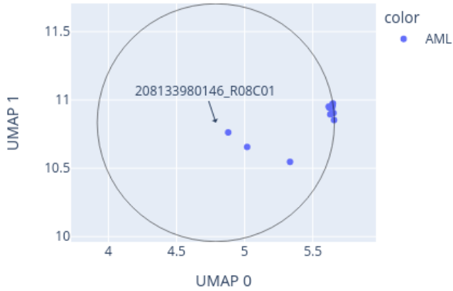
Close-up of UMAP for 208133980146_R08C01 reference: AllIDATv2_20210804_HPAP_Sarc.xlsx (19967 cases), 0 CpGs
