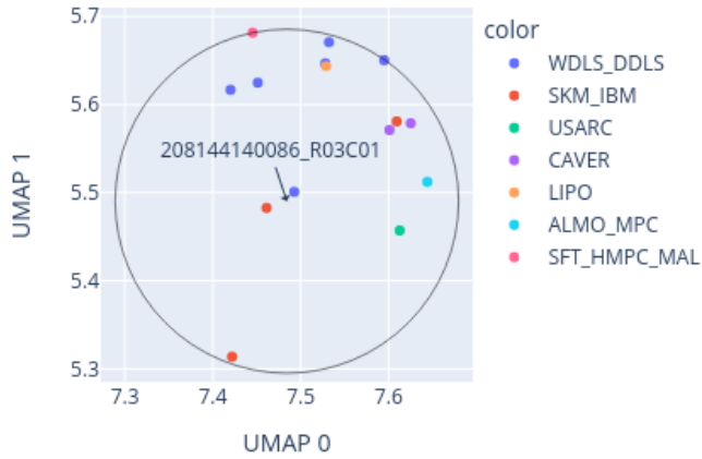
Close-up of UMAP for 208144140086_R03C01 reference: AllIDATv2_20210804_HPAP_Sarc.xlsx (19967 cases), 0 CpGs
