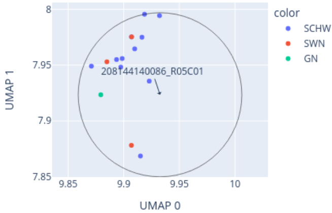
Close-up of UMAP for 208144140086_R05C01 reference: AllIDATv2_20210804_HPAP_Sarc.xlsx (19967 cases), 0 CpGs
