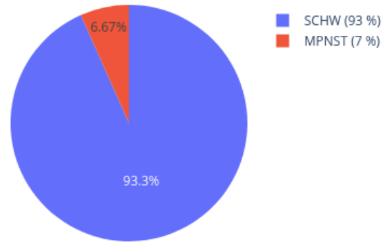
Neighbors in UMAP for 208144140086_R06C01 reference: AllIDATv2_20210804_HPAP_Sarc.xlsx (19967 cases), 0 CpGs
