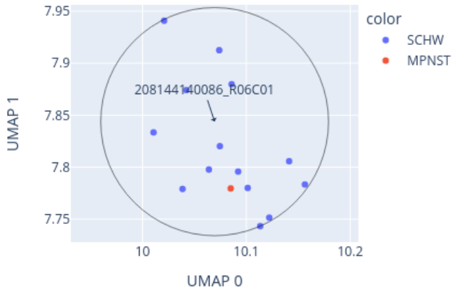
Close-up of UMAP for 208144140086_R06C01 reference: AllIDATv2_20210804_HPAP_Sarc.xlsx (19967 cases), 0 CpGs
