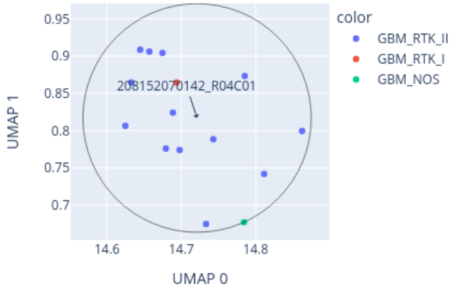
Close-up of UMAP for 208152070142_R04C01 reference: AllIDATv2_20210804_HPAP_Sarc.xlsx (19967 cases), 0 CpGs
