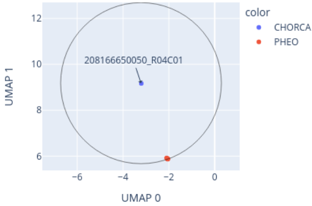
Close-up of UMAP for 208166650050_R04C01 reference: AllIDATv2_20210804_HPAP_Sarc.xlsx (19967 cases), 0 CpGs
