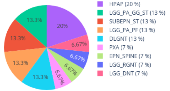
Neighbors in UMAP for 208166650075_R07C01 reference: AllIDATv2_20210804_HPAP_Sarc.xlsx (19967 cases), 0 CpGs
