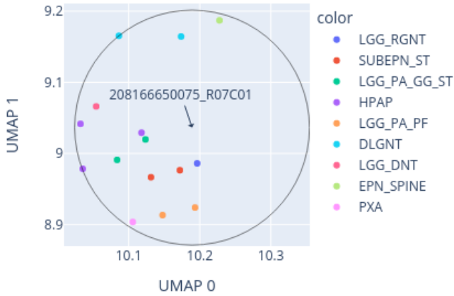
Close-up of UMAP for 208166650075_R07C01 reference: AllIDATv2_20210804_HPAP_Sarc.xlsx (19967 cases), 0 CpGs
