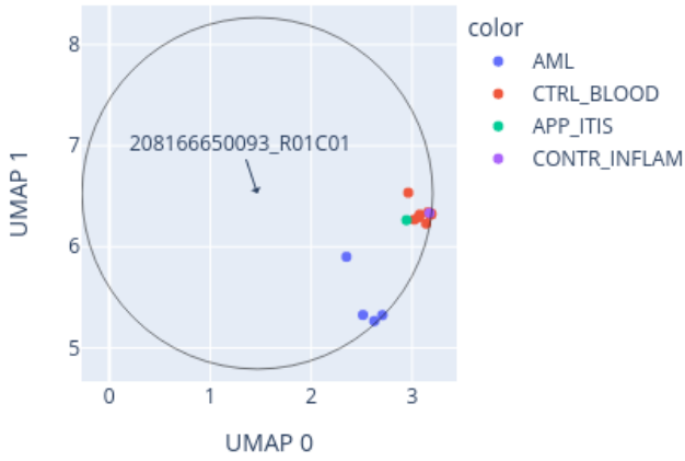
Close-up of UMAP for 208166650093_R01C01 reference: AllIDATv2_20210804_HPAP_Sarc.xlsx (19967 cases), 0 CpGs
