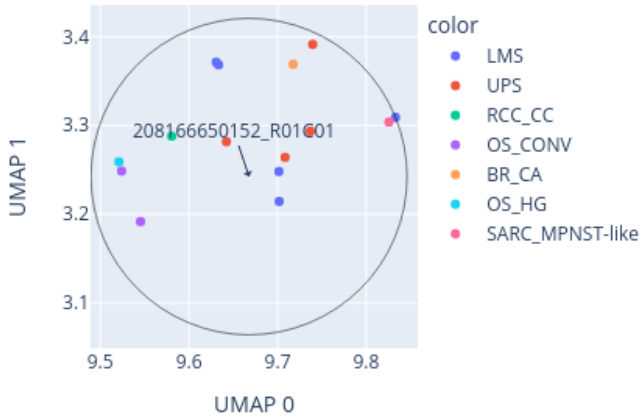
Close-up of UMAP for 208166650152_R01C01 reference: AllIDATv2_20210804_HPAP_Sarc.xlsx (19967 cases), 0 CpGs
