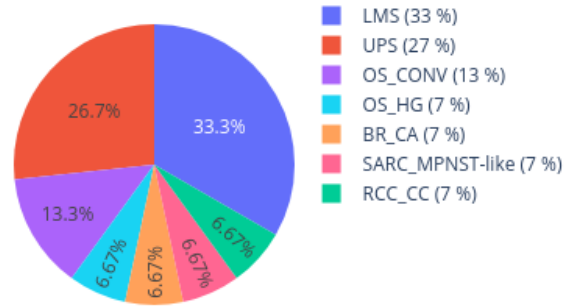
Neighbors in UMAP for 208166650152_R01C01 reference: AllIDATv2_20210804_HPAP_Sarc.xlsx (19967 cases), 0 CpGs
