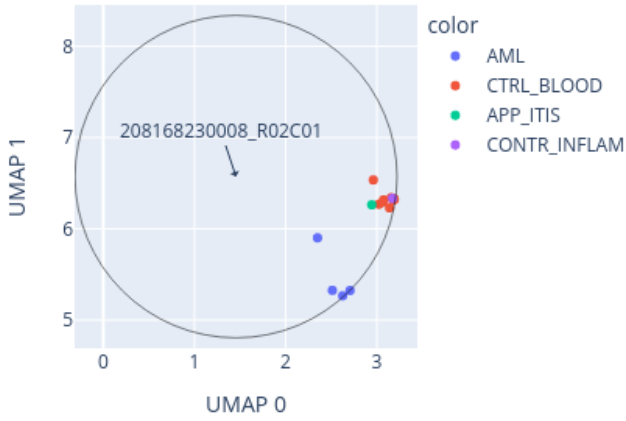
Close-up of UMAP for 208168230008_R02C01 reference: AllIDATv2_20210804_HPAP_Sarc.xlsx (19967 cases), 0 CpGs
