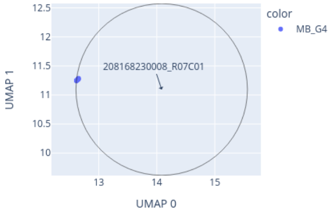
Close-up of UMAP for 208168230008_R07C01 reference: AllIDATv2_20210804_HPAP_Sarc.xlsx (19967 cases), 0 CpGs
