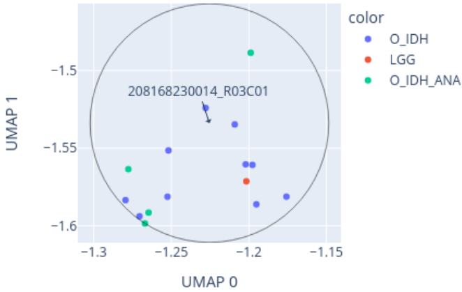
Close-up of UMAP for 208168230014_R03C01 reference: AllIDATv2_20210804_HPAP_Sarc.xlsx (19967 cases), 0 CpGs
