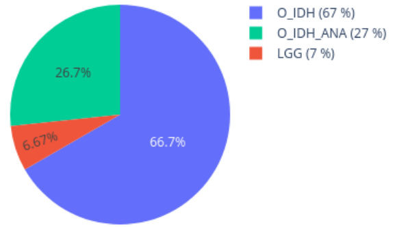
Neighbors in UMAP for 208168230014_R03C01 reference: AllIDATv2_20210804_HPAP_Sarc.xlsx (19967 cases), 0 CpGs
