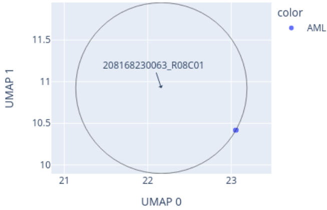
Close-up of UMAP for 208168230063_R08C01 reference: AllIDATv2_20210804_HPAP_Sarc.xlsx (19967 cases), 0 CpGs
