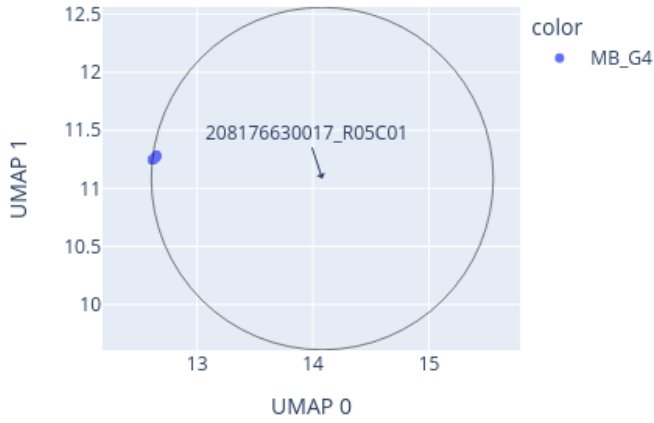
Close-up of UMAP for 208176630017_R05C01 reference: AllIDATv2_20210804_HPAP_Sarc.xlsx (19967 cases), 0 CpGs
