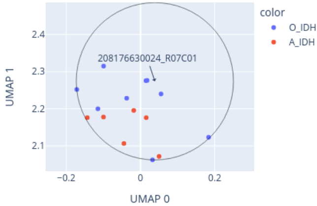
Close-up of UMAP for 208176630024_R07C01 reference: AllIDATv2_20210804_HPAP_Sarc.xlsx (19967 cases), 0 CpGs
