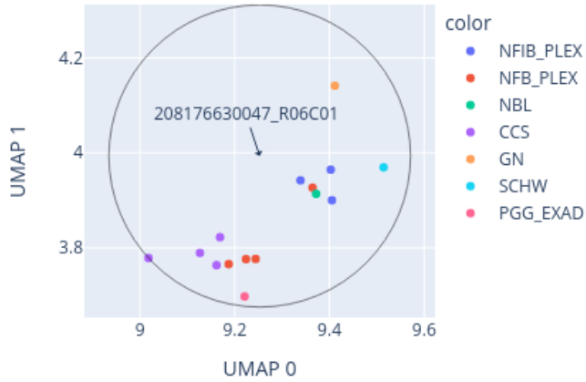
Close-up of UMAP for 208176630047_R06C01 reference: AllIDATv2_20210804_HPAP_Sarc.xlsx (19967 cases), 0 CpGs
