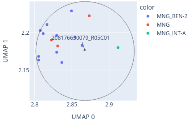
Close-up of UMAP for 208176630079_R05C01 reference: AllIDATv2_20210804_HPAP_Sarc.xlsx (19967 cases), 0 CpGs
