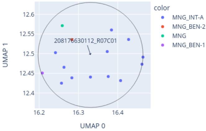
Close-up of UMAP for 208176630112_R07C01 reference: AllIDATv2_20210804_HPAP_Sarc.xlsx (19967 cases), 0 CpGs
