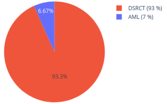
Neighbors in UMAP for 208181020077_R04C01 reference: AllIDATv2_20210804_HPAP_Sarc.xlsx (19967 cases), 0 CpGs
