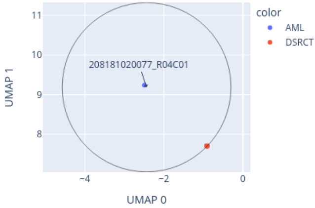
Close-up of UMAP for 208181020077_R04C01 reference: AllIDATv2_20210804_HPAP_Sarc.xlsx (19967 cases), 0 CpGs
