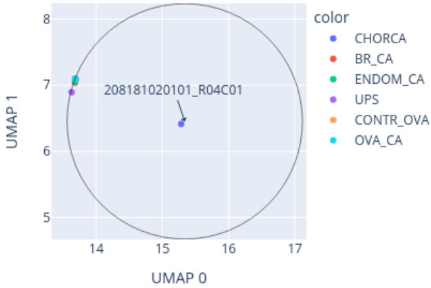
Close-up of UMAP for 208181020101_R04C01 reference: AllIDATv2_20210804_HPAP_Sarc.xlsx (19967 cases), 0 CpGs
