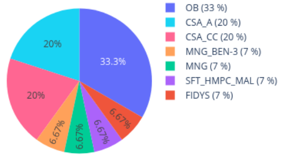
Neighbors in UMAP for 208181020103_R06C01 reference: AllIDATv2_20210804_HPAP_Sarc.xlsx (19967 cases), 0 CpGs
