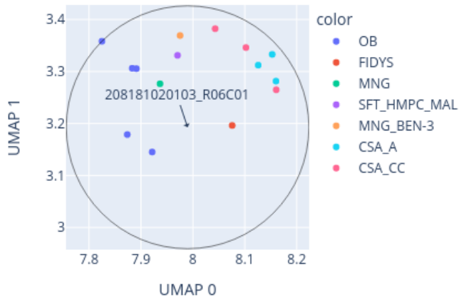
Close-up of UMAP for 208181020103_R06C01 reference: AllIDATv2_20210804_HPAP_Sarc.xlsx (19967 cases), 0 CpGs
