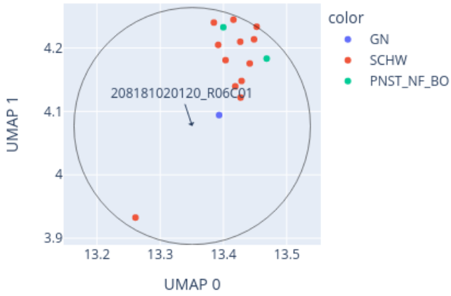
Close-up of UMAP for 208181020120_R06C01 reference: AllIDATv2_20210804_HPAP_Sarc.xlsx (19967 cases), 0 CpGs
