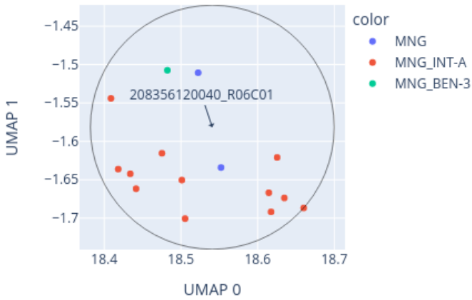
Close-up of UMAP for 208356120040_R06C01 reference: AllIDATv2_20210804_HPAP_Sarc.xlsx (19967 cases), 0 CpGs
