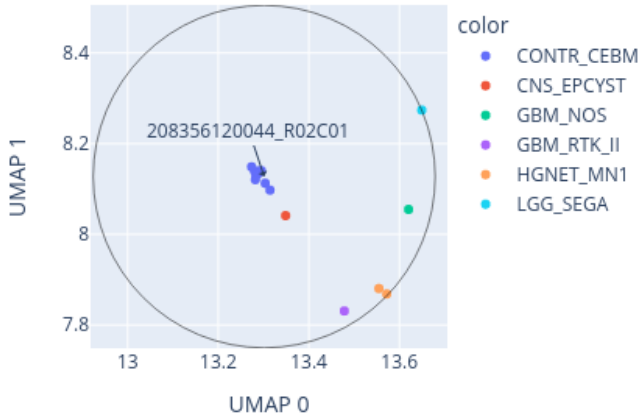
Close-up of UMAP for 208356120044_R02C01 reference: AllIDATv2_20210804_HPAP_Sarc.xlsx (19967 cases), 0 CpGs
