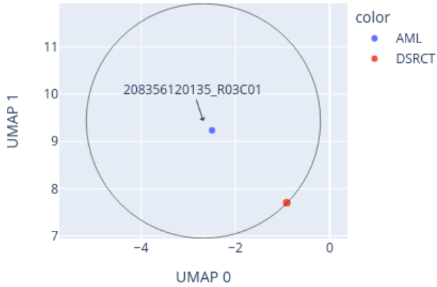
Close-up of UMAP for 208356120135_R03C01 reference: AllIDATv2_20210804_HPAP_Sarc.xlsx (19967 cases), 0 CpGs
