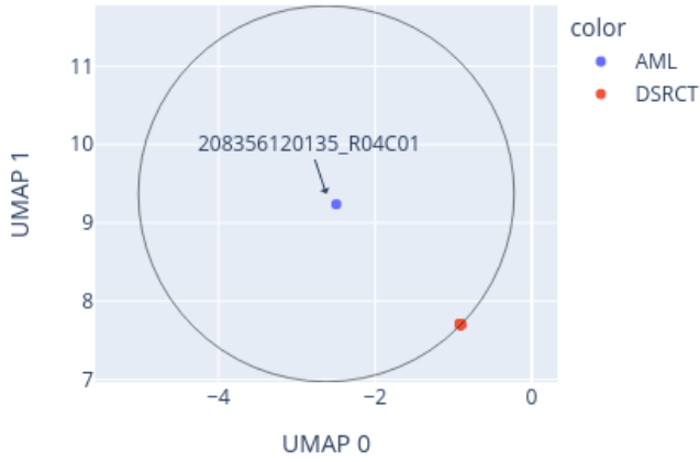
Close-up of UMAP for 208356120135_R04C01 reference: AllIDATv2_20210804_HPAP_Sarc.xlsx (19967 cases), 0 CpGs
