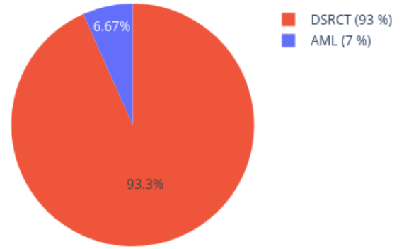
Neighbors in UMAP for 208356120135_R04C01 reference: AllIDATv2_20210804_HPAP_Sarc.xlsx (19967 cases), 0 CpGs
