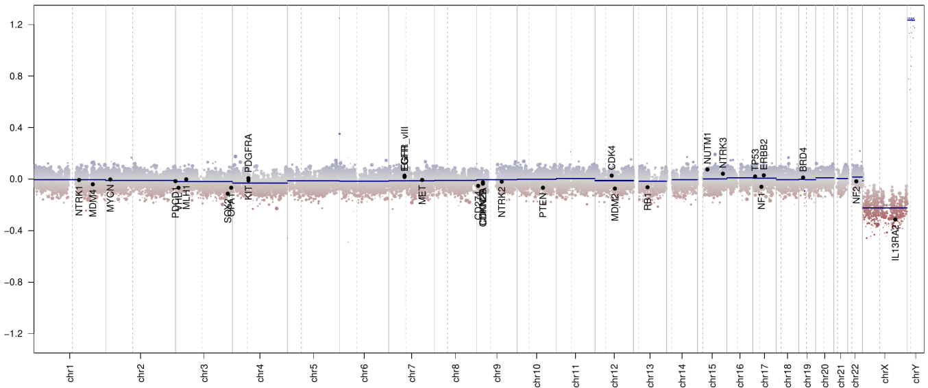
208356120152_R05C01
