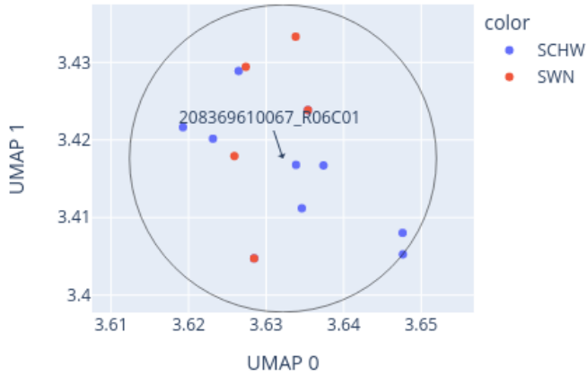
Close-up of UMAP for 208369610067_R06C01 reference: AllIDATv2_20210804_HPAP_Sarc.xlsx (19967 cases), 0 CpGs
