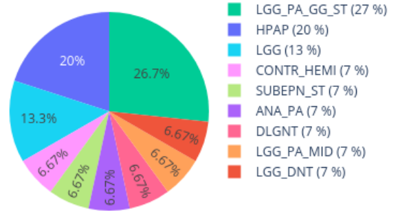
Neighbors in UMAP for 208369610067_R08C01 reference: AllIDATv2_20210804_HPAP_Sarc.xlsx (19967 cases), 0 CpGs
