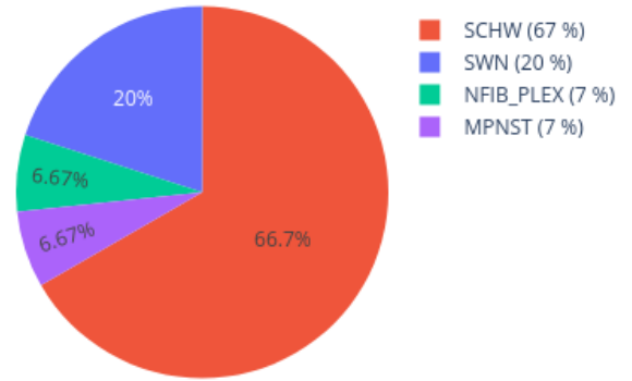
Neighbors in UMAP for 208369610069_R06C01 reference: AllIDATv2_20210804_HPAP_Sarc.xlsx (19967 cases), 0 CpGs
