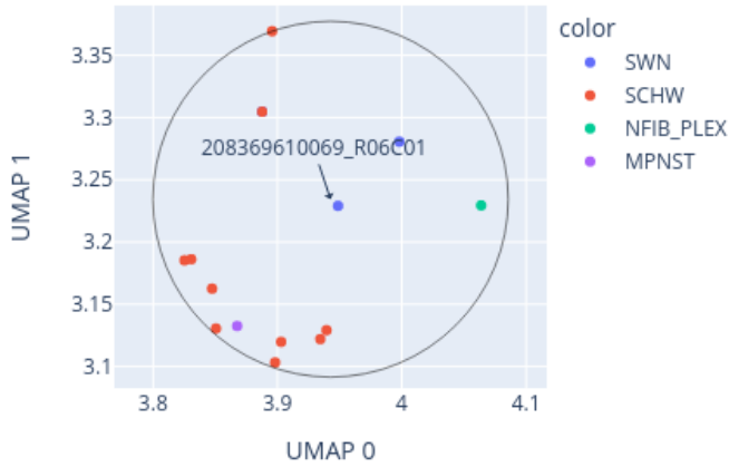
Close-up of UMAP for 208369610069_R06C01 reference: AllIDATv2_20210804_HPAP_Sarc.xlsx (19967 cases), 0 CpGs
