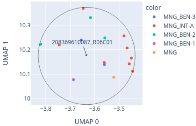
Close-up of UMAP for 208369610087_R06C01 reference: AllIDATv2_20210804_HPAP_Sarc.xlsx (19967 cases), 0 CpGs
