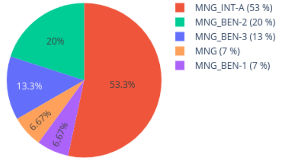
Neighbors in UMAP for 208369610087_R06C01 reference: AllIDATv2_20210804_HPAP_Sarc.xlsx (19967 cases), 0 CpGs
