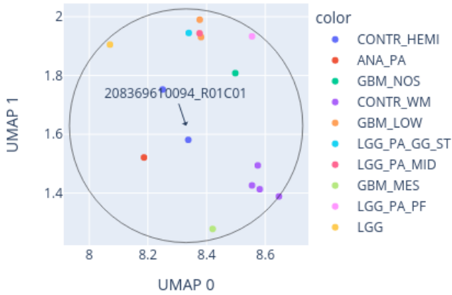
Close-up of UMAP for 208369610094_R01C01 reference: AllIDATv2_20210804_HPAP_Sarc.xlsx (19967 cases), 0 CpGs
