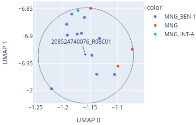
Close-up of UMAP for 208524740076_R08C01 reference: AllIDATv2_20210804_HPAP_Sarc.xlsx (19967 cases), 0 CpGs
