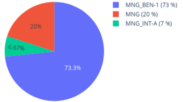
Neighbors in UMAP for 208524740076_R08C01 reference: AllIDATv2_20210804_HPAP_Sarc.xlsx (19967 cases), 0 CpGs
